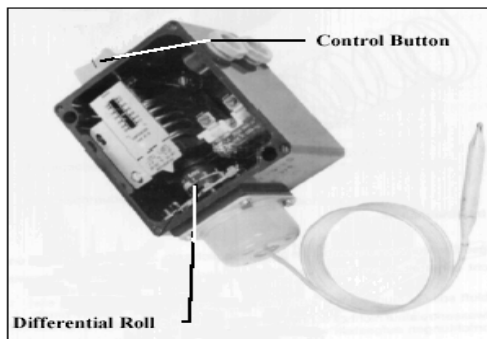
Fig. 2 One-stage thermostat RT 26
