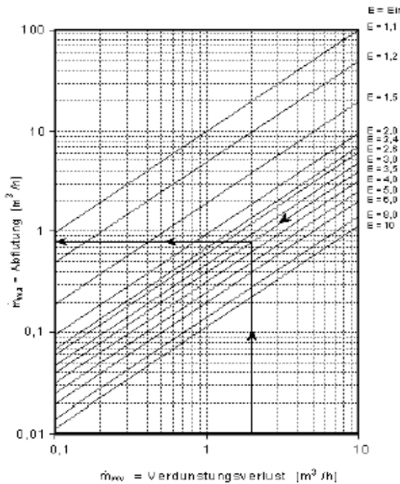
Fig. 7 Calculation of bleed-off m_{wa} depending on water concentration factor E and evaporation loss m_{wv}
