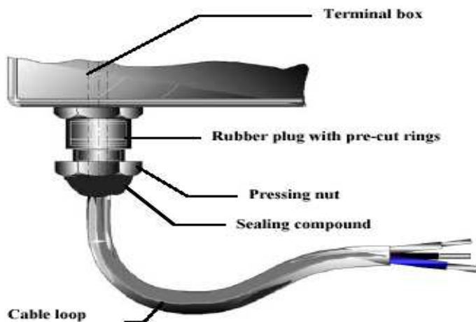
Fig.4 Sealing of Cable Inlet at Terminal Box
