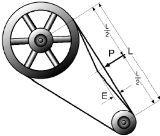
Fig.6 check V-belt tension
