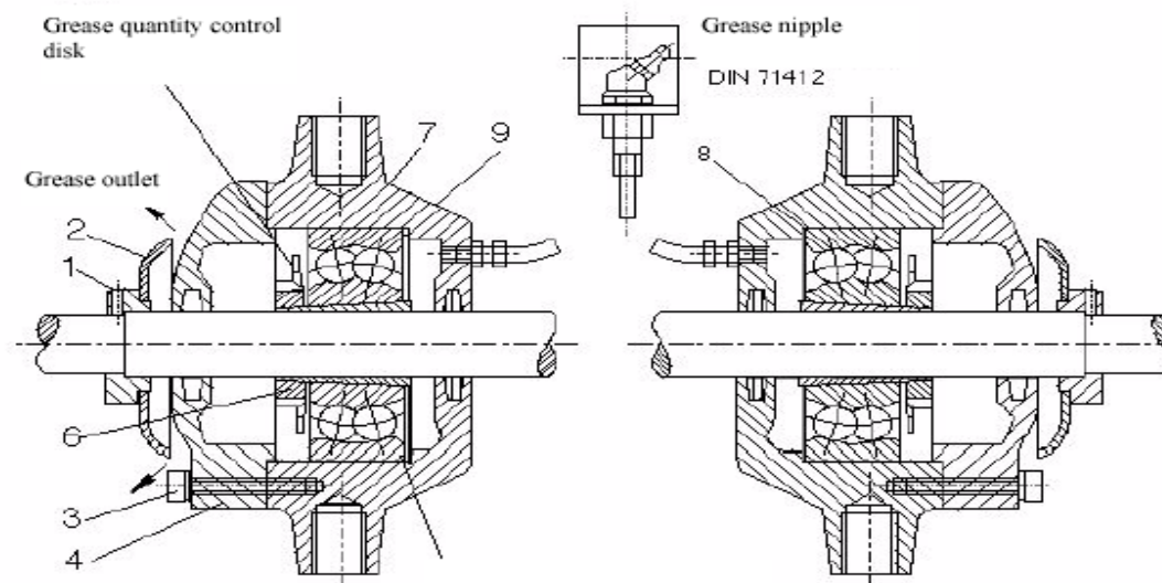
Fig.5 Self-aligning Soller bearing.
