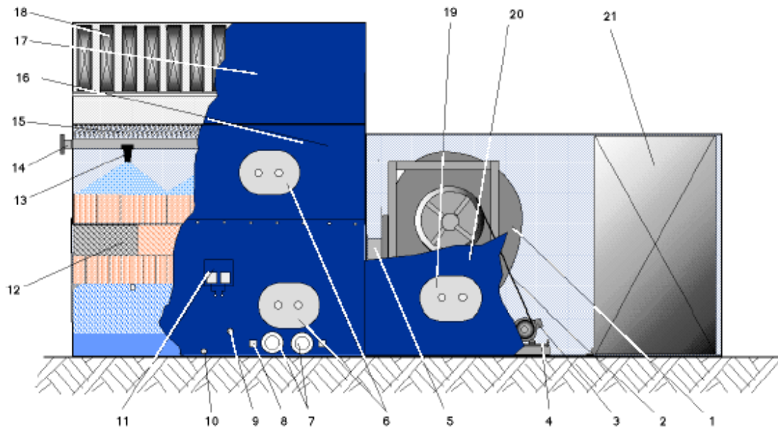
Fig. 1 Series cooling tower with torced fan arrangement, type EWK-D
